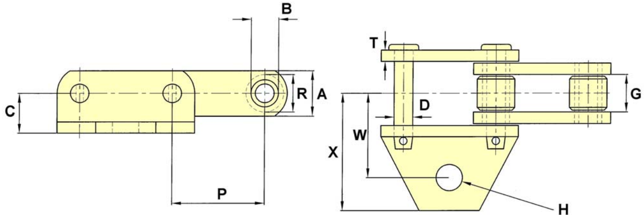
A Attachment
